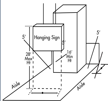
Island/Peninsula Configuration
